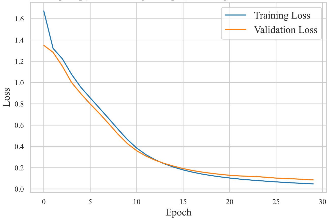
Seq2Seq (Variable-Length Output): Training and Validation Loss
